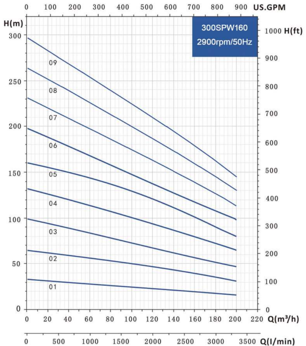
Performance Curve
